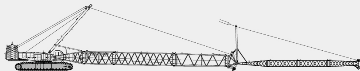
固定副臂安装示意图 Fixed Jib Installation Illustration
