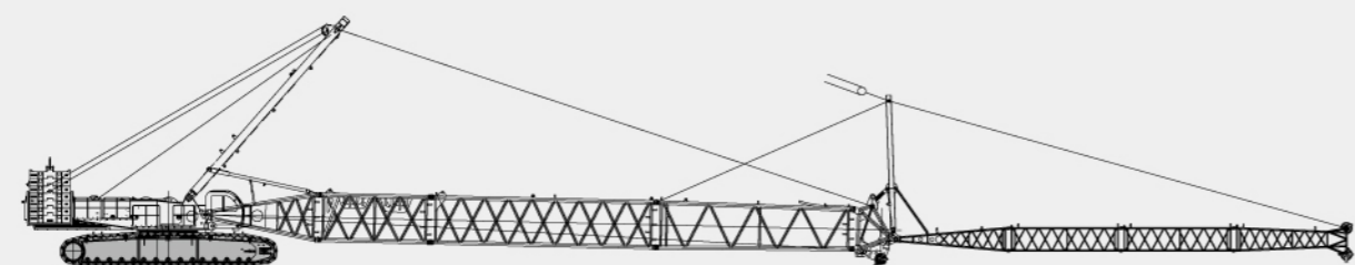
塔式副臂安装示意图 Tower Jib Installation Illustration
