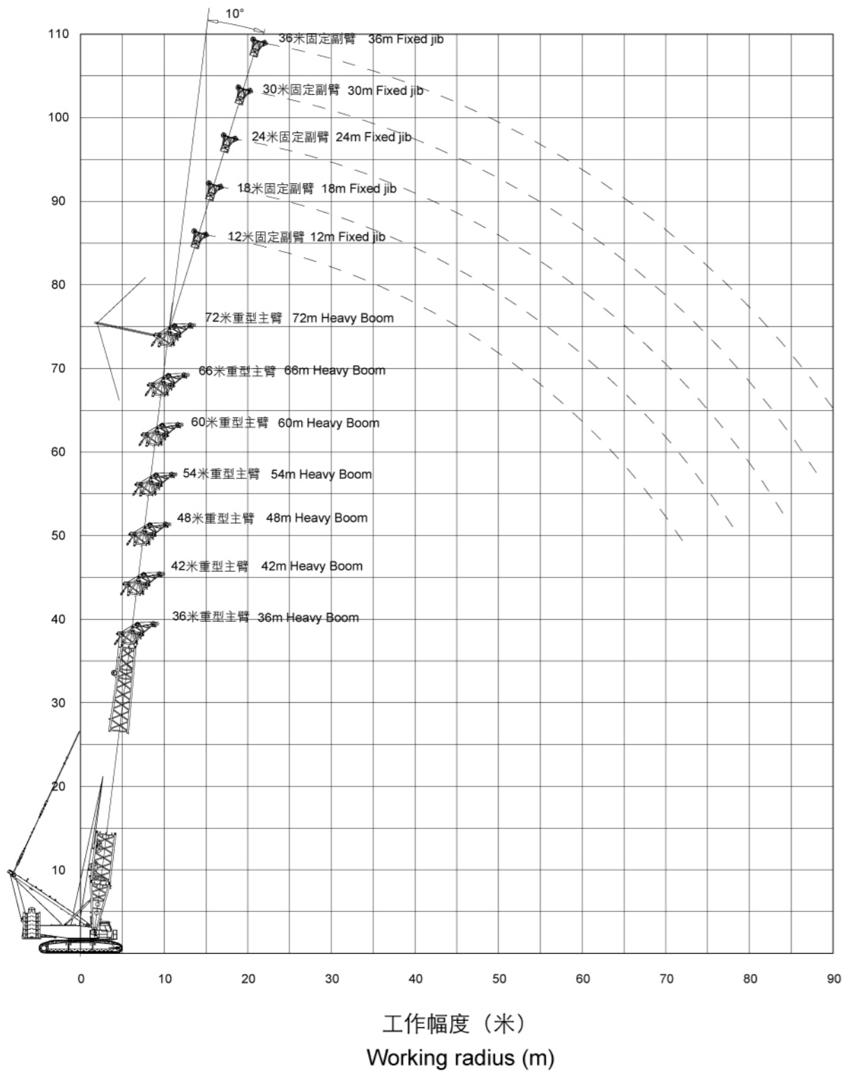
固定副臂10°时 Fixed jib angle at 10°
