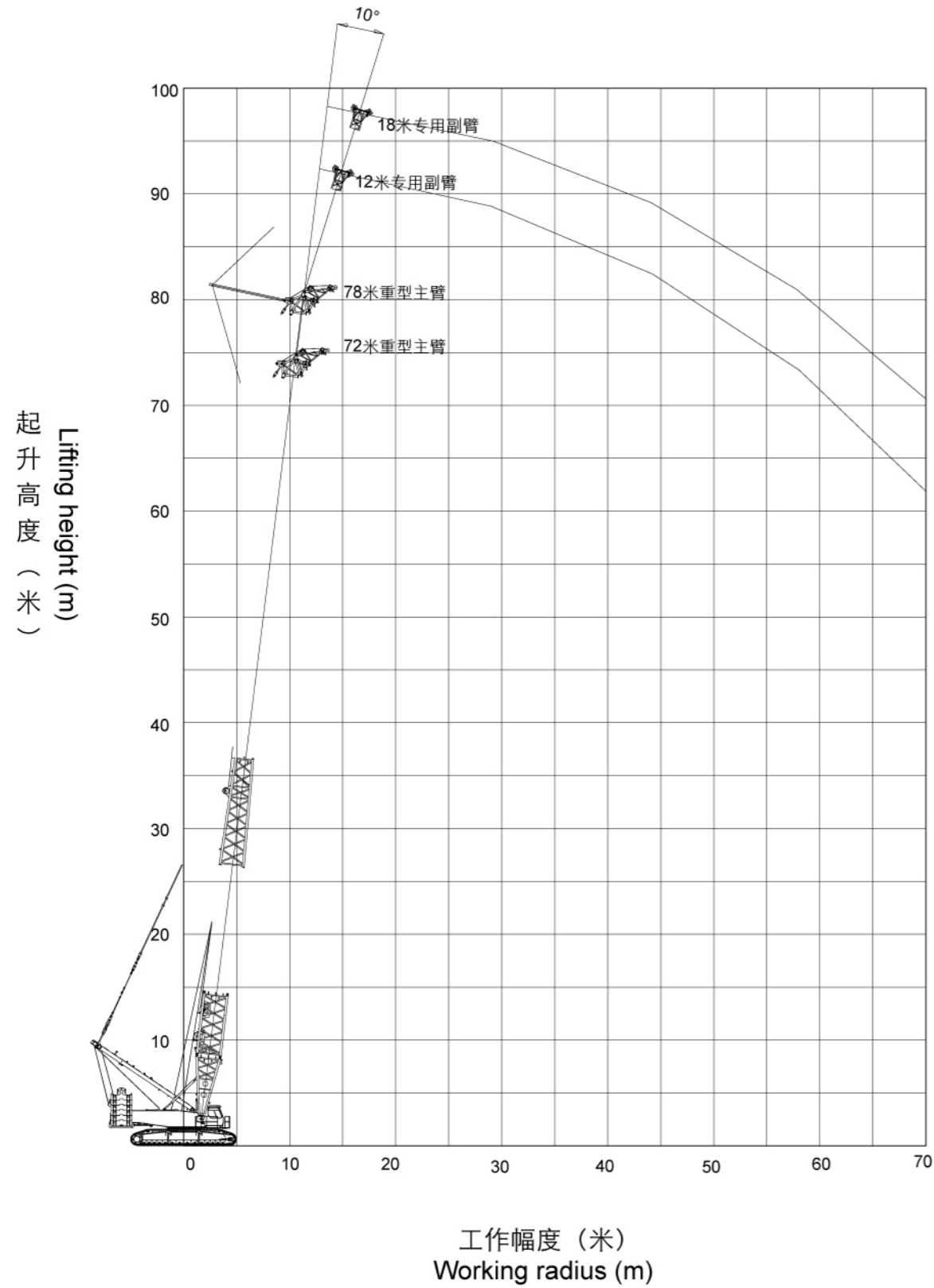
专用副臂10°时 special Jib at 10°
