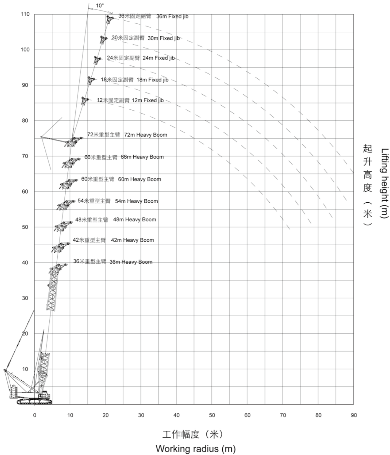
固定副臂10°时 Fixed jib angle at 10°
