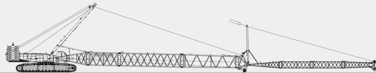
固定副臂安装示意图 Fixed Jib Installation Illustration
