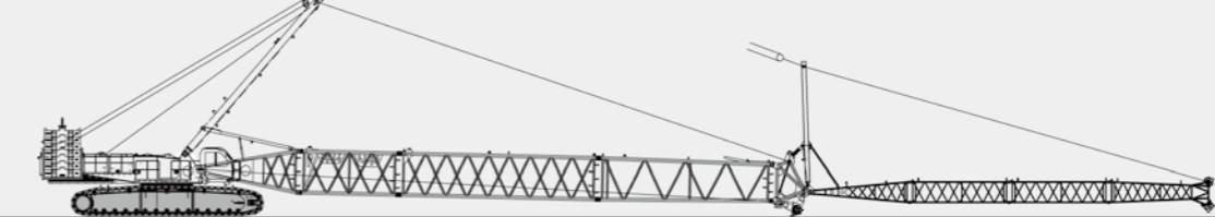
固定副臂安装示意图 Fixed Jib Installation Illustration
