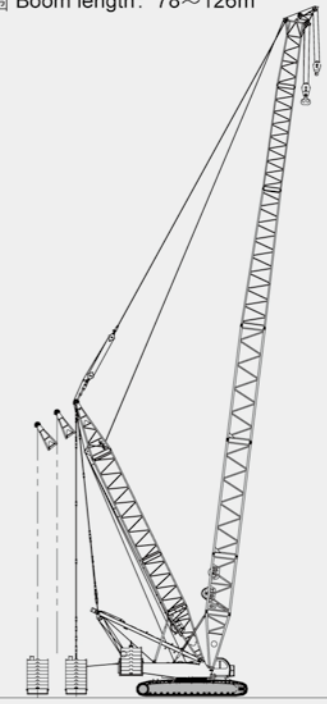
标准工况专用副臂 Standard Mode Special Jib
